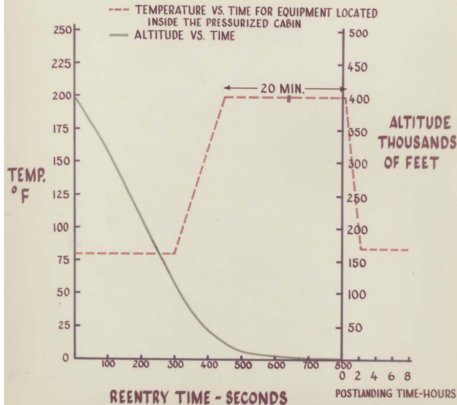
CURVE I TEMPERATURE-ALTITUDE PROFILE FOR REENTRY
